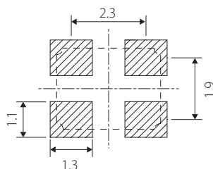
Land Pattern(REFERENCE)
