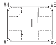
Land Pattern(REFERENCE)
