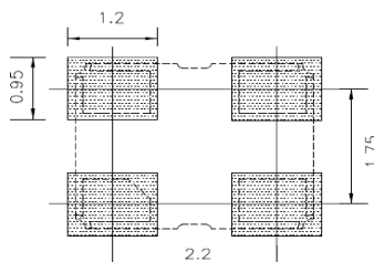
Land Pattern(REFERENCE)
