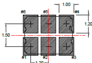
Land Pattern(REFERENCE)
