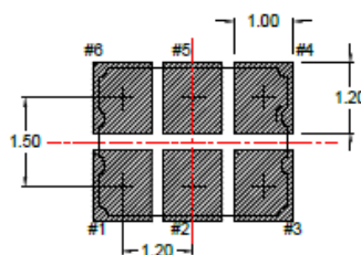
Land Pattern(REFERENCE)
