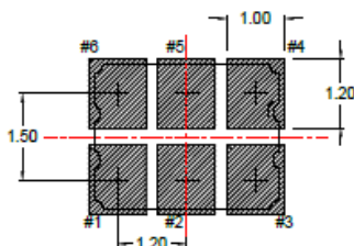
Land Pattern(REFERENCE)
