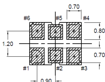
Land Pattern(REFERENCE)
