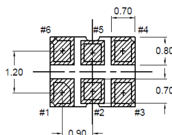
Land Pattern(REFERENCE)
