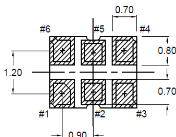
Land Pattern(REFERENCE)
