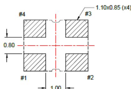
LAND PATTERN (REFERENCE)
